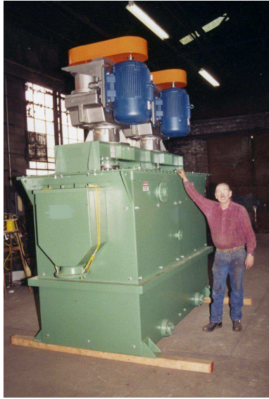
48" x 48" Duplex Attrition Scrubber lined with abrasion resistant plate
